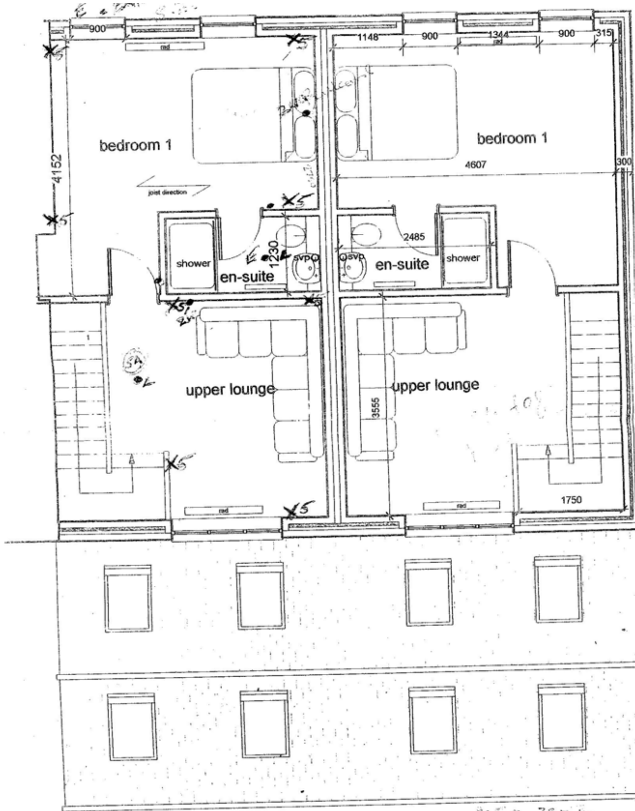
Proposed Layout Plan -First Floor
